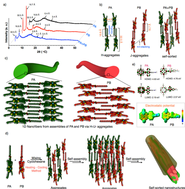
Fig. 4 (a) Powder X-ray diffraction analysis of PA, PB and PA + PB. (b) Molecular packing of PA, PB, and PA + PB leading to H, J-aggregates and self-sorted from the corresponding d -spacing values for each length of the center to the end, \pi - \pi stacking, and H-bonding. (c) Schematic representation of the self-assembly in PA and PB, leading to the formation of 1D nanofibers. (d) Schematic illustration of the formation of self-sorted nanostructures by mixing PA + PB via self-assembly. (e) Optimized structures and the corresponding HOMO/LUMO energy levels of PA and PB from DFT calculations. The electrostatic potential maps of PA and PB exhibit the charge distribution.
