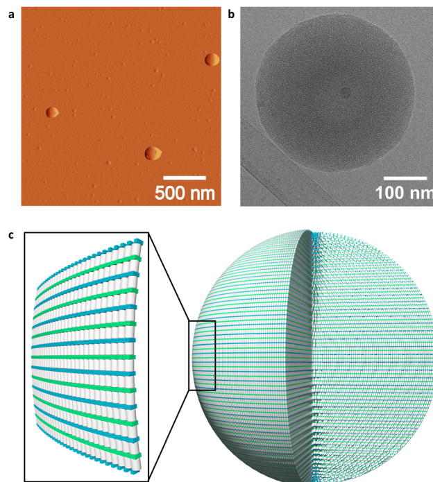
Fig. 3 (a) AFM deflection image of 1*2 deposited on APTES-modified mica, (b) cryo-EM image of 1*2 , and (c) illustration of a self-assembled 1*2 nanoparticle and zoom-in on outermost layer (DNA in grey, 2,7-dialkynyl phenanthrene 2,7-Ph in blue, and 3,6-dialkynyl phenanthrene \alpha in green). Conditions: 1 \mu M 1*2 , 10 mM sodium phosphate buffer pH 7.2, 0.10 mM spermine tetrahydrochloride, and 20 vol% ethanol.
