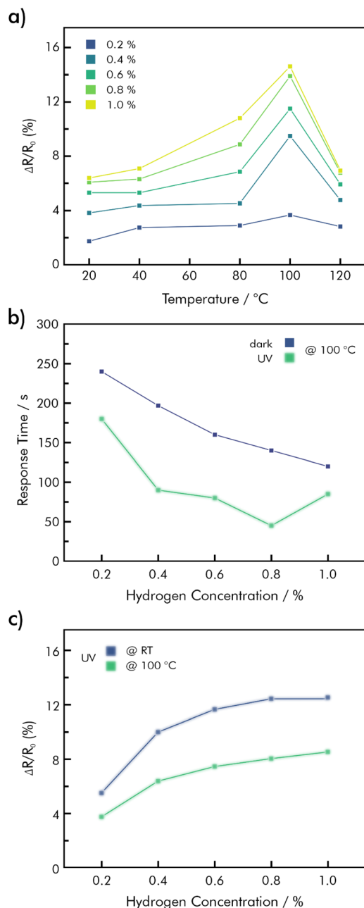
Fig. 11 Hybrid Pd/rGO sensing performance (a) temperature-dependent responses towards \text{H}_2 at different concentrations; (b) effect of UV-illumination on response times as a function of \text{H}_2 -concentration at 100 ^{\circ}\text{C} ; (c) signal responses under UV-illumination at RT and 100 ^{\circ}\text{C} as a function of \text{H}_2 -concentration; redrawn with data from ref. 82.
