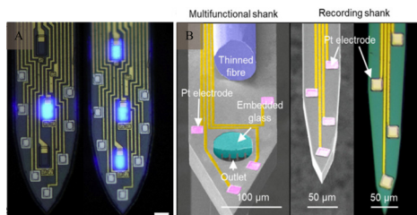
Fig. 7 Optical probes and injectable optoelectronics. (A) High-magnification images of the illuminated micro light-emitting diodes (scale bar: 15 μm). Reproduced with permission from ref. 74. (B) A multifunctional, implantable optoelectronic device. Reproduced with permission from ref. 75.
