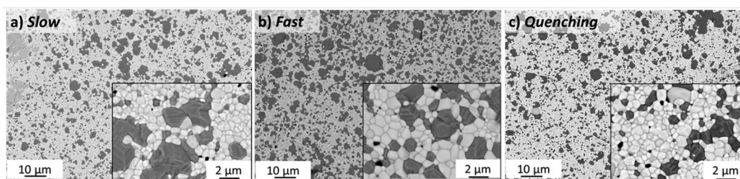
Fig. 8 BSE-images of surface morphology of 60CGO20–FCO subjected to different heat treatment in the furnace at (a) 1200 °C for 100 h and subsequent 850 °C for 100 h with standard cooling; (b) 1200 °C for 100 h with free cooling in air (c) 1200 °C for 100 h with quenching in water.
