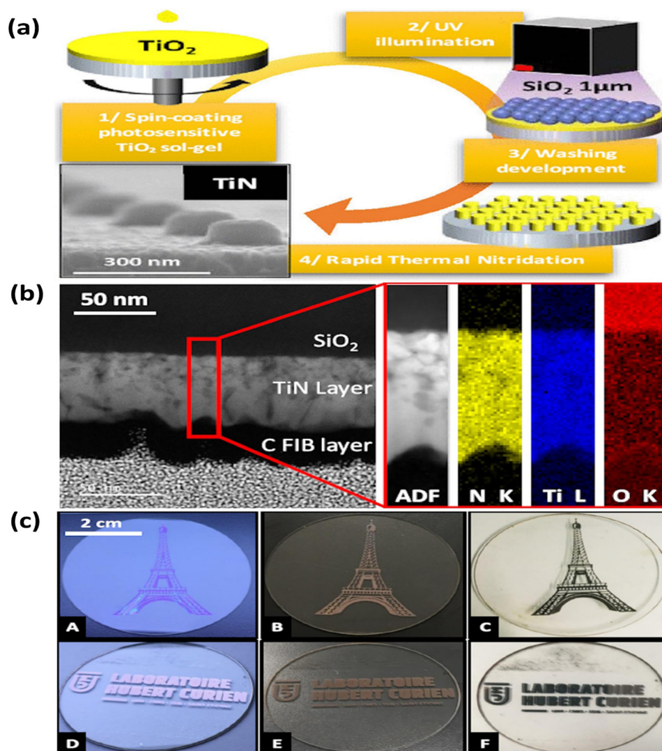
Fig. 8 (a) Scheme for the preparation; (b) cross-sectional HRTEM of the \text{TiN} thin film, annular dark field (ADF), and element mapping images for the N, Ti, and O; (c) photographs of structured \text{TiO}_2 thin films after UV exposure (A) and (D), after nitridation (B) and (E) and in transmission (C) and (F) elements in the \text{TiN} layer (reproduced from ref. 109 with permission).
