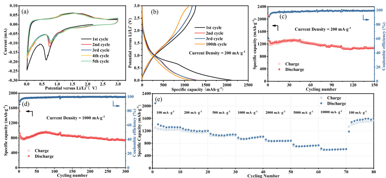
Fig. 4 The CV curves for the initial 5 cycles (a), and charge and discharge voltage profile (b) of the Fe 3 O 4 QDs@C/RGO composite. Cycling performance under a low current density of 200 mA g -1 (c), long-term lithium-ion storage capability under a current density of 1000 mA g -1 (d), and rate capability (e) of the Fe 3 O 4 QDs@C/RGO composite.
