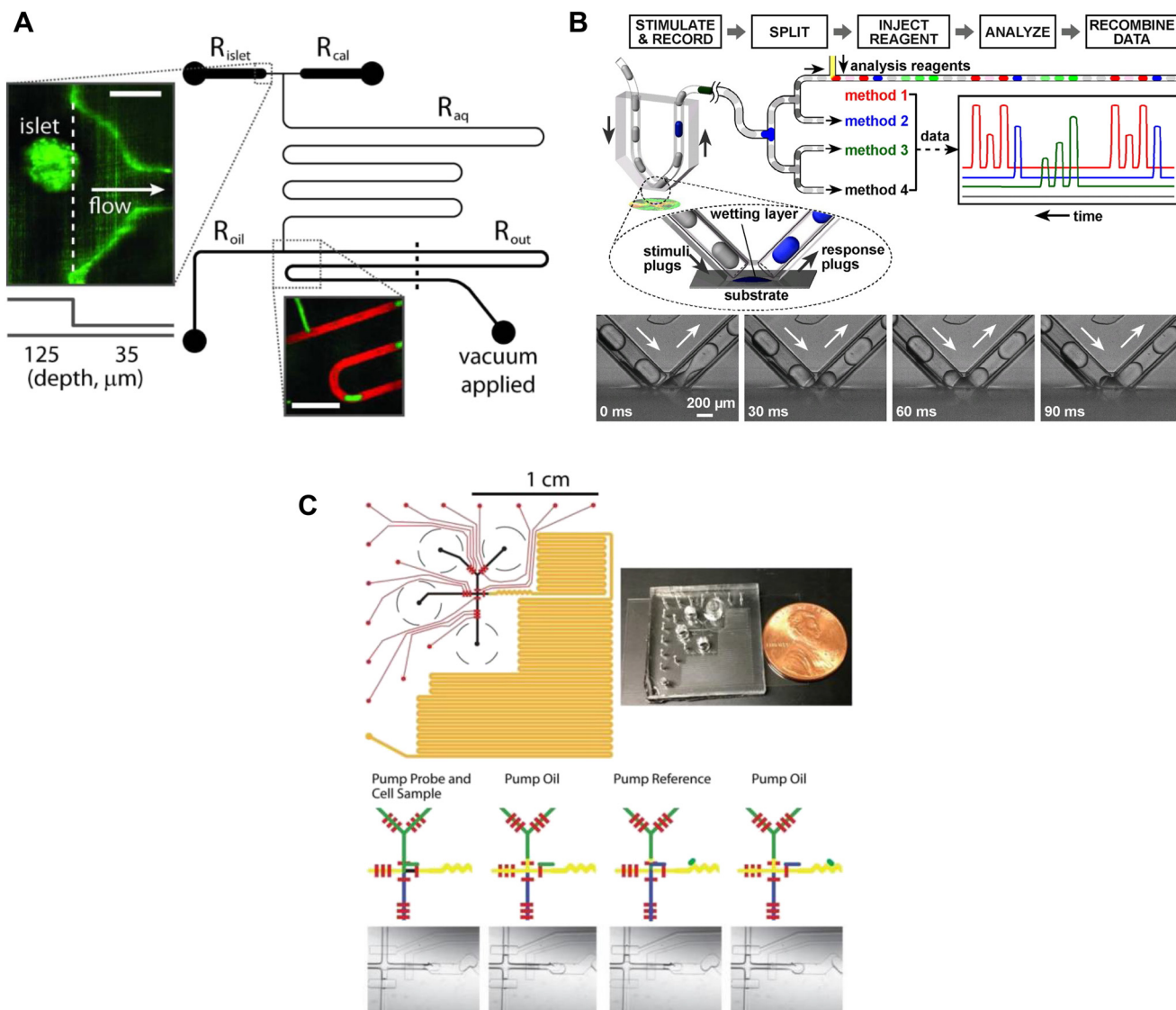
Fig. 4 Examples of droplet microfluidic devices to measure insulin secretion from individual islets. A) Islets were continuously perfused with treatment and FluoZin-3 through R_{islet} . Droplets of islet effluent with FluoZin-3 are formed downstream of R_{oil} and sequentially stored for analysis in R_{out} . R_{cal} inlet was primarily used as a vacuum inlet to introduce stimulation or for calibration measurements of FluoZin-3. Reproduced with permission from ref. 56. B) A droplet microfluidic device that used surface wetting of droplets to sample islet effluent. The droplets were then injected with immunoassay reagents for subsequent insulin quantification by FCS measurement. Islets sat in a stimulant buffer within a MatTek dish. © 2008 by the National Academy of Sciences of the USA. Reproduced with permission from ref. 57. C) A droplet microfluidic device with a long incubation channel (orange) to store and image droplets after incubation time has been met. The black circles represent the reservoirs for the islet, oil, probe and reference. The red channels represent the pneumatic control channels that automate the chip operation. Reproduced with permission from ref. 59.
