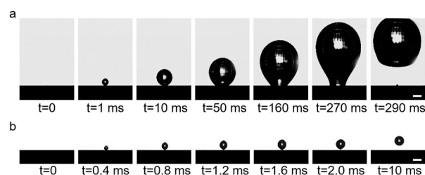
Fig. 3 Processes of bubble formation in the (a) adsorption state and (b) desorption state in 1 mmol \text{L}^{-1} SDS solution. Scale, 500 \mu\text{m} .
