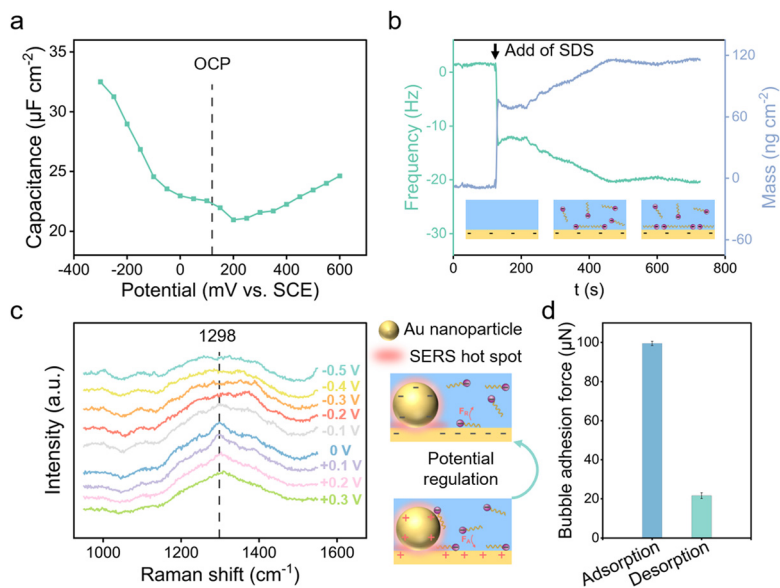
Fig. 2 Adsorption and desorption of anionic surfactants on the Au surface. (a) Differential capacitance of the Au surface in 1 mmol \text{L}^{-1} \text{NaClO}_4 solution. The minimum value, approximately 0.20 V, corresponds to the potential of zero charge ( E_{\text{PZC}} ). Meanwhile, the open circuit potential ( E_{\text{OCP}} ) value of about 0.12 V is negative than the E_{\text{PZC}} value, indicating a negatively charged surface under open circuit conditions; (b) change in frequency of Au-coated quartz crystal sensor upon adsorption of \text{DS}^- on the surface in 1 mmol \text{L}^{-1} SDS solution; (c) SERS spectra of the Au nanoparticle-coated Au electrode at different electrode potentials. The peak at 1298 \text{cm}^{-1} (originating from the dodecyl tail of \text{DS}^- ) disappeared when the potential was negative than -0.2 V, indicating the desorption of \text{DS}^- from the surface due to electrostatic repulsion; (d) the bubble adhesion force of surface in the adsorption and desorption states.
