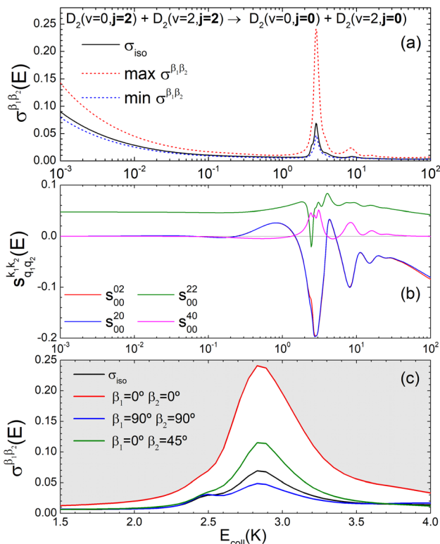
Fig. 5 (a) Isotropic cross section (solid black curve) as a function of E_{\text{coll}} for D_2(v=0, j=2) + D_2(v=2, j=2) \rightarrow D_2(v=0, j=0) + D_2(v=2, j=0) collisions. The maximum and minimum values of the cross sections that could be achieved by a given alignment of the two internuclear axes of the diatoms are shown as red and blue dashed curves, respectively. (b) The relevant s_{q_1q_2}^{k_1k_2} as a function of E_{\text{coll}} . (c) \sigma^{\beta_1\beta_2} calculated as a function of E_{\text{coll}} for the four given preparations. The region above the maximum value of the cross section that could be achieved is shaded in grey.
