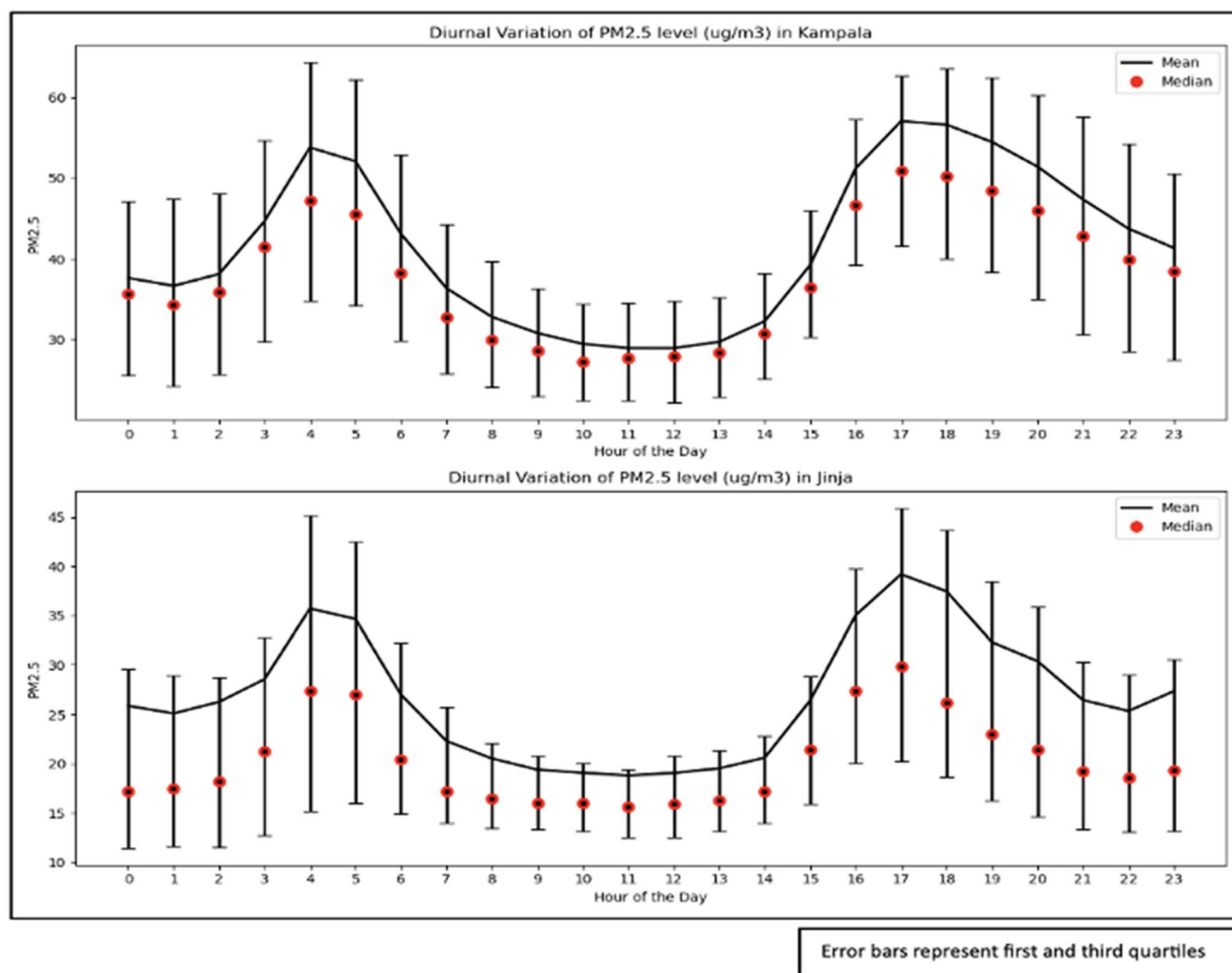
Fig. 3 Diurnal variation of PM 2.5 (μg m -3 ) in Kampala and Jinja.
