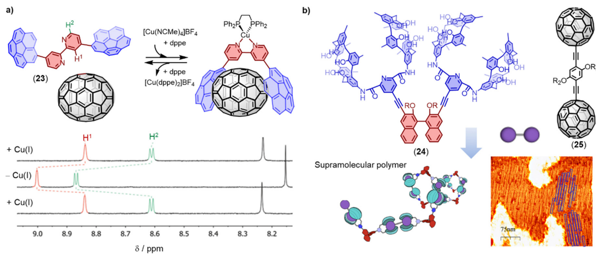
Fig. 12 (a) Chemical structure of 2,2'-bipyridine-bridged molecular tweezers 23 and its in situ coordination/decoordination of C 70 as monitored using 1 H-NMR in CD 2 Cl 2 at 298 K. Adapted from ref. 176 with permission from Royal Society of Chemistry, Copyright 2021. (b) Schematic representation of the formation of supramolecular polymers based on bis(salicyl)arenes tweezers 24 and dumbbell fullerenes 25 . Adapted from ref. 177 with permission from American Chemical Society, copyright 2021.
