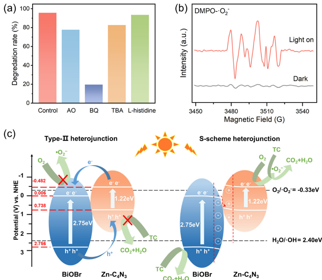
Fig. 7 (a) Trapping experiments of active species about the photocatalytic degradation of TC. (b) ESR spectra of DMPO- \cdot\text{O}_2^- in methanol dispersions over Zn- \text{C}_4\text{N}_3 /BiOBr after irradiation. (c) Possible photocatalytic mechanism for Zn- \text{C}_4\text{N}_3 /BiOBr.
