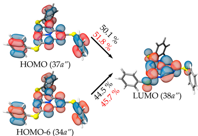
Fig. 7 Molecular orbitals and their contributions to the S_1 ( T_1 in red) transition calculated at the ADC(2)/def2-TZVP level of theory for molecule 1 .
