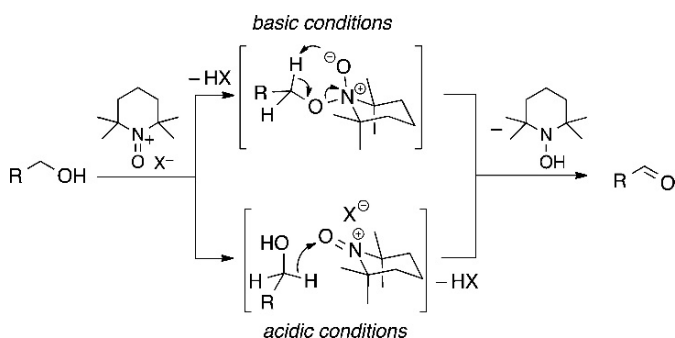
Figure 4. Projected alcohol oxidation driven by TEMPO + /TEMPOH couple in different conditions towards aldehyde. Copyright: M. Rafiee, K. C. Miles and S. S. Stahl, J. Am. Chem. Soc. , 2015, 137 , 14751-14757.
