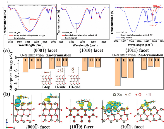
Figure 10. IR absorption of different ZnO nanomaterial before and after BnOH adsorption. The range is focused on the O–H stretch. (a): Calculated absorption energy of benzyl alcohol in different facets on different facets of ZnO hexagons. (b): electron density prediction of varied facets of ZnO with adsorbed benzyl alcohol. Credit: H.
