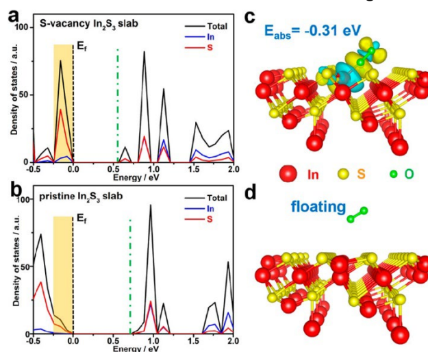
Figure 18. (a), (b): DFT calculated DOS for In 2 S 3 slabs with and without S-vacancy. (c), (d): Illustration of simulated O 2 interaction with both slabs. Credits: X. Sun, L. Sun, X. Zhang, J. Xie, S. Jin, H. Wang, X. Zheng, X. Wu and Y. Xie. J. Am. Chem. Soc. , 2019, 141, 9, 3797–3801.
