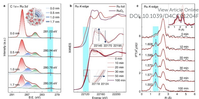
Figure 17. (a) XPS data at varied depths of the material. (b) in situ XANES spectra recorded at Ru K-edge during heating process. (c) in situ EXAFS spectra recorded during heating process. Inset: overlay of EXAFS region among the different time points. Credit: D. Liu, T. Ding, L. Wang, H. Zhang, L. Xu, B. Pang, X. Liu, H. Wang, J. Wang, K. Wu and T. Yao, Nat. Commun. , 2023, 14, 1, 1720
