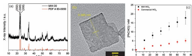
Figure 12. (Left) X-ray Diffraction data and (centre) TEM imaging of the obtained microwave synthesized \text{WO}_3 ; (right) Concentration of benzaldehyde, oxidation product of benzyl alcohol, over time during \text{WO}_3 photocatalysis. Black squares: microwave synthesized nanoplatelets; Red circles: commercial material. Credit: K. D. McDonald and B. M. Bartlett, RSC Adv. , 2019, 9, 28688-28694.
