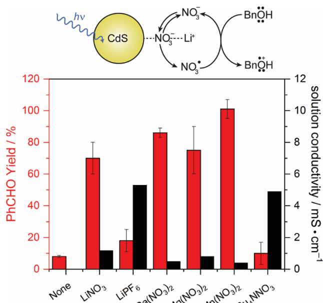
Figure 6. (Top) Proposed mechanism of nitrate mediated benzyl alcohol oxidation with \text{LiNO}_3 as a mediator. (Down) Yield of benzaldehyde after 48h irradiation with CdS and 50 mM mediator listed. Error bars represent deviations among 3 trials. Copyright: J. L. DiMeglio, A. G. Breuhaus-Alvarez, S. Li and B. M. Bartlett, ACS Catal., 2019, 9, 5732-5741.
