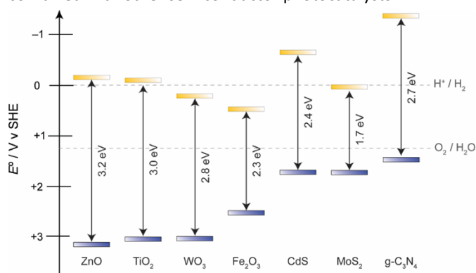
Figure 1. Band edge positions of noble-metal free photocatalysts highlighted in this review.
