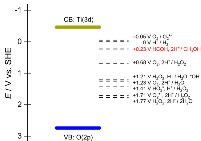
Figure 2. Standard potentials involving active oxygen species superimposed on the band edges of \text{TiO}_2 .
