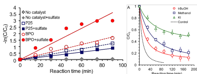
Figure 7. Rate comparison of 2,4-DCP oxidation under varied conditions. Left: with or without sulfate on BPO/P25- \text{TiO}_2 ; Right: with or without radical scavengers. Copyright: G. Liu, S. You, Y. Tan and N. Ren, Environ. Sci. Technol., 2017, 51, 2339-2346.
