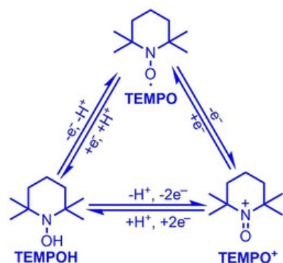
Figure 3. Electron and proton transfer of TEMPO-TEMPO + -TEMPOH conversion. Copyright: X. Lang and J. Zhao, Chem. Asian J. , 2018, 13 , 599-613.
