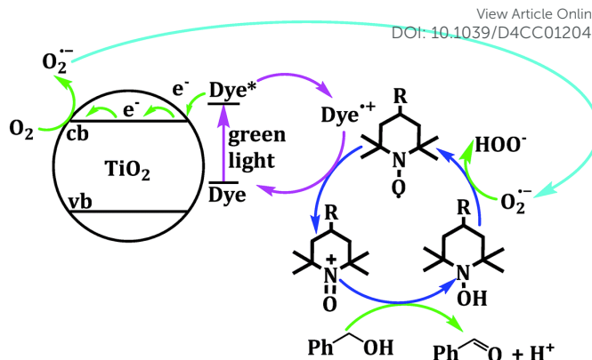
Figure 5. Proposed mechanism of TEMPO-derivative driven benzyl alcohol oxidation on dye-sensitized TiO 2 . Copyright: N. Wang, J. L. Shi, H. Hao, H. Yuan and X. Lang, Sustainable Energy Fuels , 2019, 3 , 1701-1712
