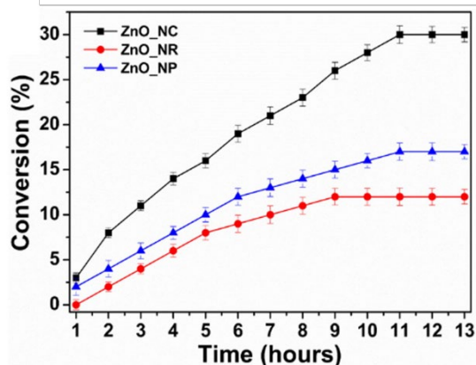
Figure 9. Percentage conversion of benzyl alcohol oxidation reaction over time powered by UV light under aerobic conditions with different shaped ZnO nanomaterials. Credit: H. Weerathunga, C. Tang, A. J. Brock, S. Sarina, T. Wang, Q. Liu, H. Y. Zhu, A. Du and E. R. Waclawik, J. Colloid Interface Sci. , 2022, 606 , 588-599.
