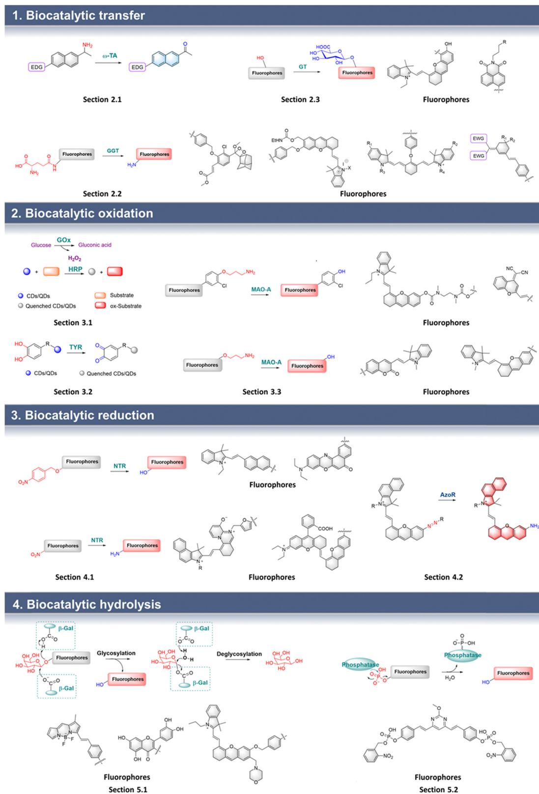
Fig. 1 Fluorescent probes for biocatalysts.
