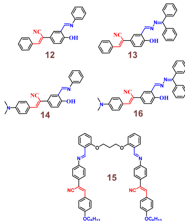
Fig. 19 Chemical structure of probe 12–16 .
