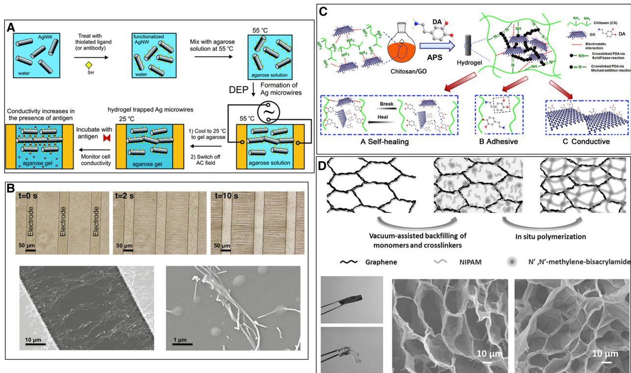
Fig. 14 Processing methods to increase electrical conductivity of nanocomposite hydrogels. (A) Functionalized silver nanowires in warm water–agarose solution aligned through dielectrophoresis (DEP). After cooling down, agarose gelation occurs and a hydrogel with anisotropic electrical conductivity is formed. The conductivity increases in the presence of antigen due to the tighter packing of the functionalized silver nanowires. Reproduced from ref. 60 with permission from The Royal Society of Chemistry. (B) Nanocomposite hydrogel with chitosan, polydopamine and reduced GO. Self-healing mechanism attributable to the electrostatic interactions between GO and chitosan and the non-covalent bonding of catechol groups. Adhesiveness as a result of the catechol groups of polydopamine. Electrical conductivity through the reduced GO. Reprinted from ref. 119, Copyright 2016, with permission from Elsevier. Dielectrophoretic alignment of CNT between electrode bands. Phase images of CNT dielectrophoretic alignment over time. SEM images of dielectrophoretically aligned CNTs between two electrodes. Reprinted from ref. 167, Copyright 2017, with permission from Elsevier. (D) Graphene monolith – poly- N -isopropylacrylamide hydrogel. Photos of nanocomposite (dark and rigid) and pristine (transparent) hydrogel and SEM images of graphene monolith and freeze-dried nanocomposite hydrogel. Reprinted with permission from ref. 114. Copyright 2014 Wiley.
