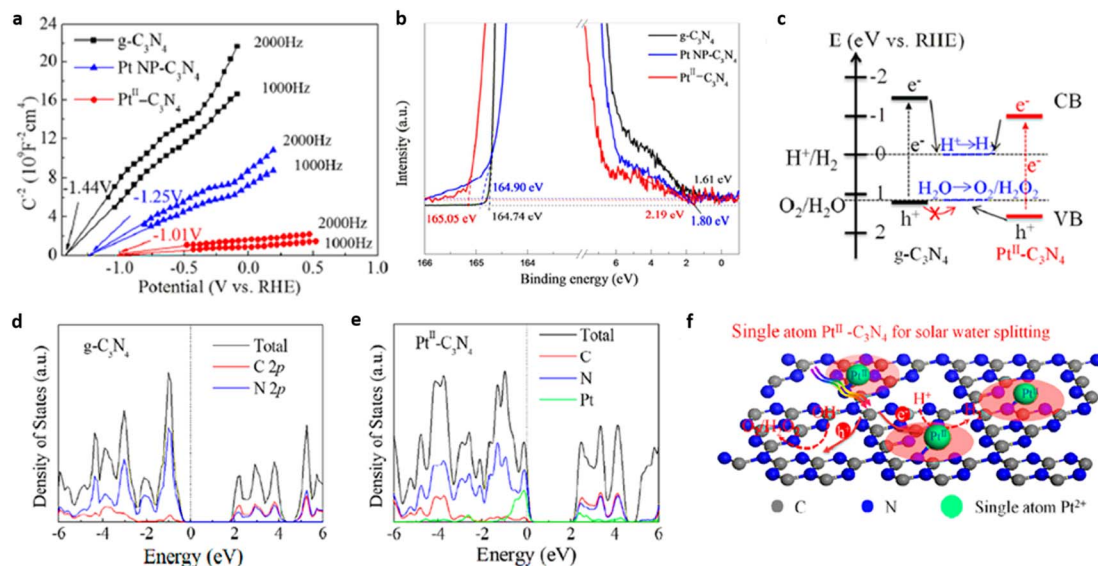
Fig. 18 (a) Mott–Schottky plot of \text{Pt}^{\text{II}}-\text{C}_3\text{N}_4 in comparison with g-\text{C}_3\text{N}_4 and \text{Pt NP}-\text{C}_3\text{N}_4 , (b) UPS spectra of g-\text{C}_3\text{N}_4 , \text{Pt}^{\text{II}}-\text{C}_3\text{N}_4 & \text{Pt NP}-\text{C}_3\text{N}_4 , (c) schematic band structure alignment, DOS of (d) g-\text{C}_3\text{N}_4 and (e) \text{Pt}^{\text{II}}-\text{C}_3\text{N}_4 , (f) mechanistic pathways (schematic) of the photocatalytic water splitting by \text{Pt}^{\text{II}}-\text{C}_3\text{N}_4 . Reproduced with permission from ref. 23. Copyright 2018 American Chemical Society.
