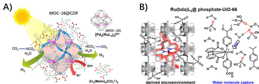
Fig. 12 The uptake of (A) carbonate in MOC-16@ZIF-8 and (B) phosphate in \text{Ru}(\text{bda})\text{L}_2 @UiO-66 (reproduced from ref. 76 with permission from Elsevier), as a proton mediator/relay to assist the proton delivery through a hydrogen-bond network of water molecules.
