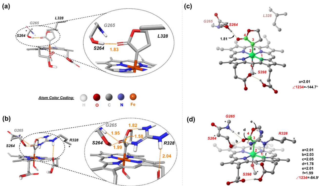
Fig. 4 Lowest-energy structures of the metalcarbene intermediate of the H-bonding pattern seen in the lowest energy structures of (a) C^{L9} and (b) C^{L10} . DFT optimized structures of (c) C^{L9} and (d) C^{L10} . The H atoms (except the ones taking part in H-bonding) are omitted for clarity. The dashed orange lines represent H-bonding. Distances are in Å.
