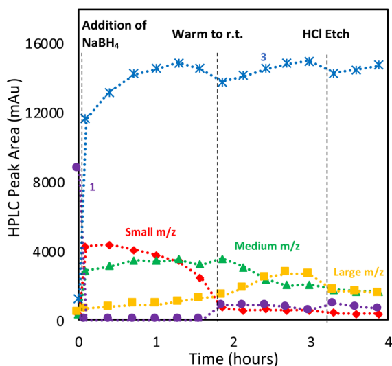
Fig. 3 HPLC monitoring of major products and regional analysis size regions in the synthesis of (4). Blue star (3), red diamond (small region), green triangle (medium region), yellow square (large region), purple circle (1). The first data point after the zero point was obtained 1 minute after addition of NaBH 4 .
