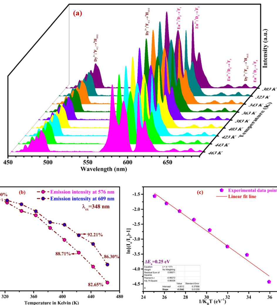
Fig. 11 (a) Temperature-dependent PL spectra of NDE1 phosphor under 348 nm excitation wavelength (b) relative intensity vs. temperature plot for emission peak wavelengths at 576 and 609 nm for NDE1 phosphor under 348 nm excitation wavelength (c) plot of \ln((I_0/I_T) - 1) vs. 1/K_B T ( \text{eV}^{-1} ) for NDE1 phosphor.
