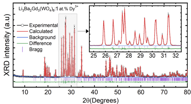
Fig. 2 Rietveld refinement plots for \text{Li}_3\text{Ba}_2\text{Gd}_3(\text{WO}_4)_8:1 \text{ at}\% \text{Dy}^{3+} : the experimental profile—black line; the calculated pattern—red line; the difference plot—green line and the background—blue line; (Inset) zoomed view in the range between 25 and 32°.
