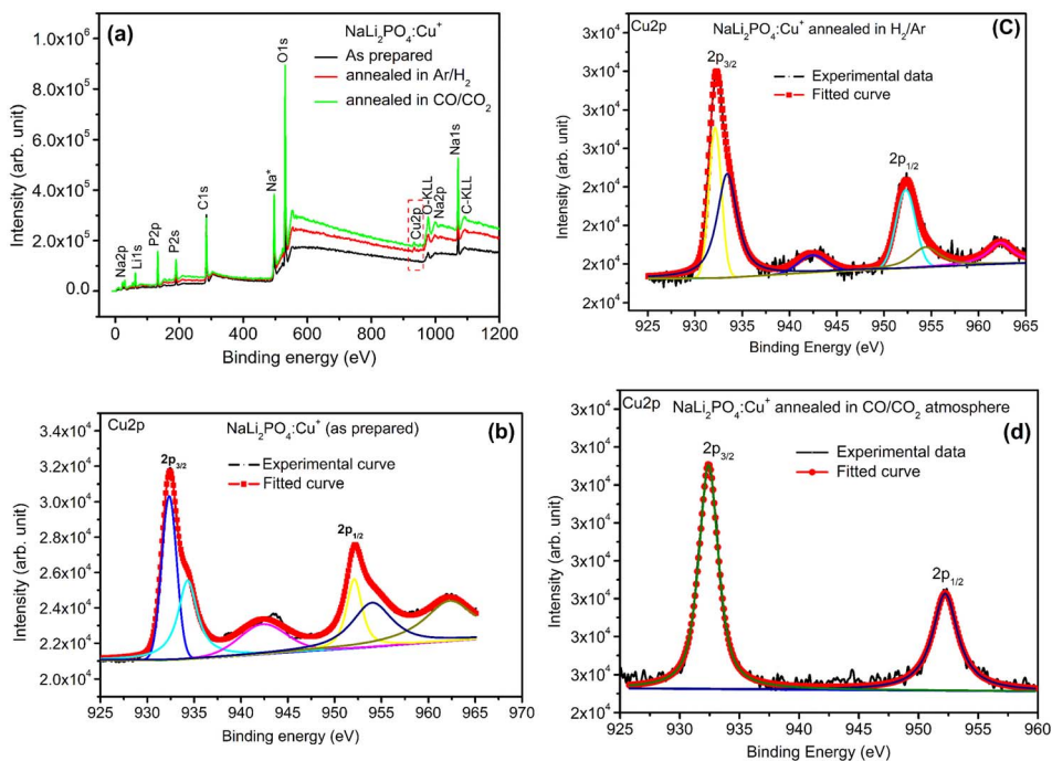
Fig. 9 (a) XPS survey of \text{NaLi}_2\text{PO}_4:\text{Cu}(\text{I}) annealed in various atmospheres for Cu ions, (b) XPS deconvoluted spectrum of \text{NaLi}_2\text{PO}_4:\text{Cu}(\text{I}) as prepared sample for Cu 2p_{3/2} and Cu 2p_{1/2} , (c) XPS spectrum of \text{NaLi}_2\text{PO}_4:\text{Cu}(\text{I}) annealed in 10% \text{H}_2 in Ar atmosphere at 400 °C for Cu 2p_{3/2} and Cu 2p_{1/2} , (d) XPS spectrum of \text{NaLi}_2\text{PO}_4:\text{Cu}(\text{I}) annealed in \text{CO}/\text{CO}_2 atmosphere at 800 °C for Cu 2p_{3/2} and Cu 2p_{1/2} .
