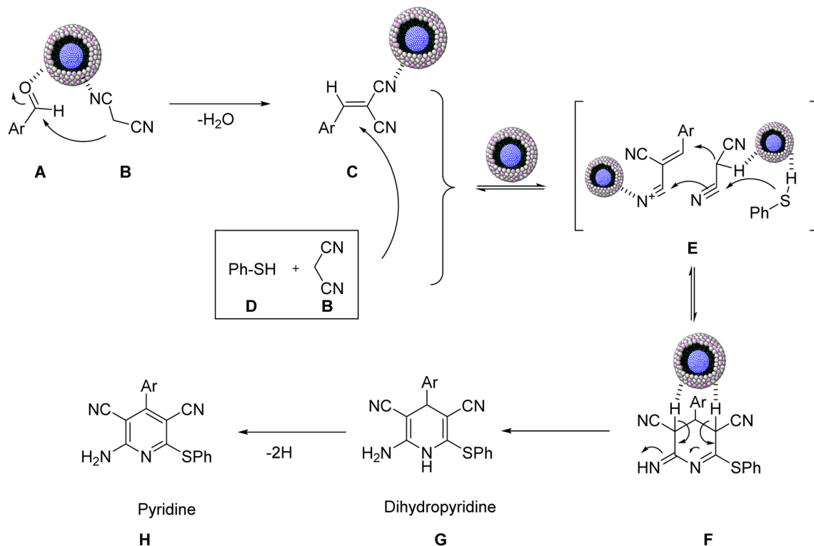
Scheme 6 Plausible mechanism for the construction of substituted pyridine derivatives catalyzed by \text{Ni}^{\text{II}} -picolyamine/TCT/APTES@ \text{SiO}_2@\text{Fe}_3\text{O}_4 .
