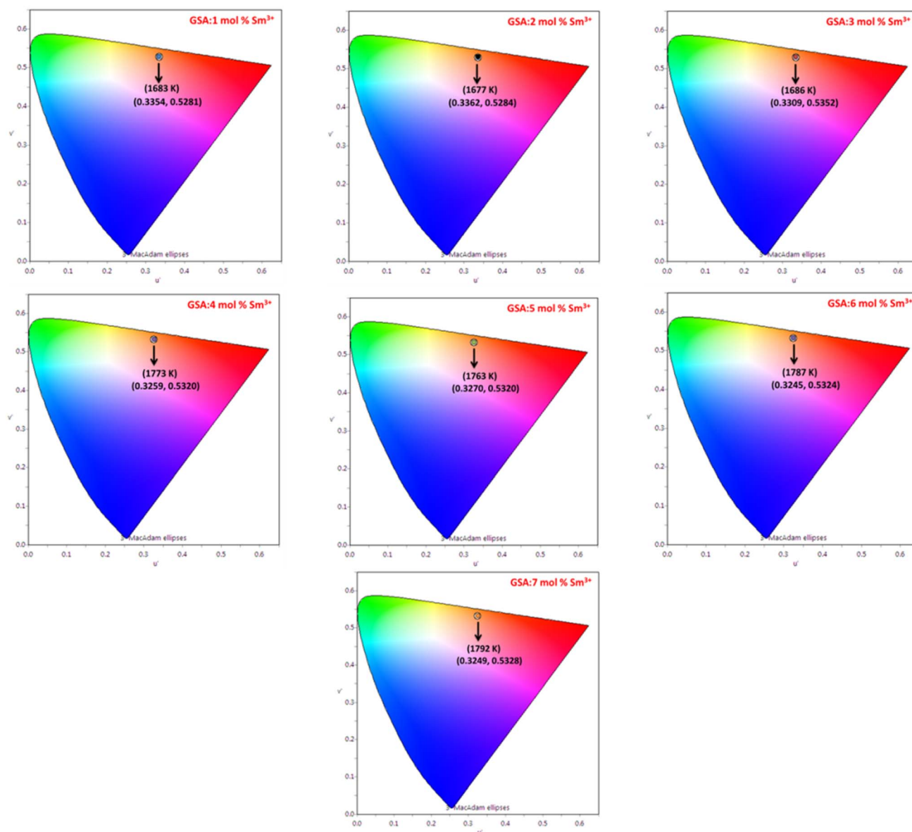
Fig. 18 Representation of u' , v' with CCT values of Gd_{1-x}Sr_2AlO_5:x \text{ mol\% } Sm^{3+} (1–7 mol%) phosphors.
