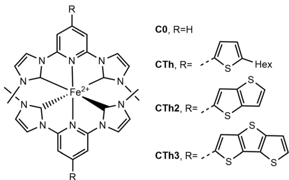
Fig. 2 Complexes studied in this work. The counterion is PF 6 - throughout.
