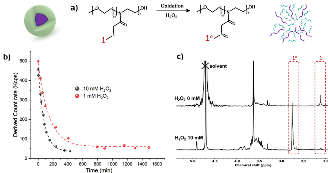
Fig. 7 (a) Schematic illustration of the oxidative reaction of PEG- b -PMTMeOx (DP = 30) block copolymer NPs with H_2O_2 , (b) decrease of DLS scattering light intensity of the nanoparticle solution at 1 \text{ mg mL}^{-1} when adding 1 and 10 mM H_2O_2 and (c) ^1H NMR spectra of PEG- b -PMTMeOx before and 24 hours after oxidation with 10 mM H_2O_2 in D_2O .
