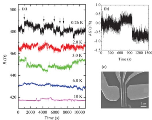
Fig. 16 (a) Resistance at five temperatures for a \text{RuO}_2 NW with length L = 1.5 \mu\text{m} and diameter d = 67 \text{ nm} . Data at 6.0 K, 3.0 K, 2.0 K, and 0.26 K are offset by 10 \Omega , 20 \Omega , 30 \Omega , and 40 \Omega , respectively, for clarity. (b) Conductance variation \delta G = G - \langle G \rangle vs. time at 0.26 K. (c) Scanning electron microscope (SEM) image of lithographically defined NW. Reproduced from ref. 65 with permission. Copyright 2011 American Institute of Physics.
