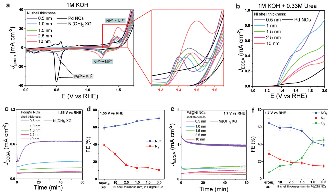
Fig. 2 The electrochemical performance of Pd@Ni NCs. (a) CV recorded at 20 \text{mV s}^{-1} scan rate at Pd@Ni NCs with different shell thickness, Pd NCs and Ni(OH) 2 xerogel in 1 M KOH. (b) ECSA-normalised anodic sweeps of CV recorded at 20 \text{mV s}^{-1} scan rate at Pd@Ni NCs with different shell thickness and Pd NCs in 1 M KOH containing 0.33 M urea. ECSA was determined based on the Ni redox peak surface area in 1 M KOH for Pd@Ni NCs and using CO stripping method for Pd NCs. (c) ECSA-normalised chronoamperometry curves (c and e) and FEs of the major products of 0.33 M urea electrolysis (d and f) in 1 M KOH performed at 1.55 V (c and d) and 1.7 V (e and f) using Pd@Ni NCs with different shell thickness or Ni(OH) 2 xerogel as the anode.
