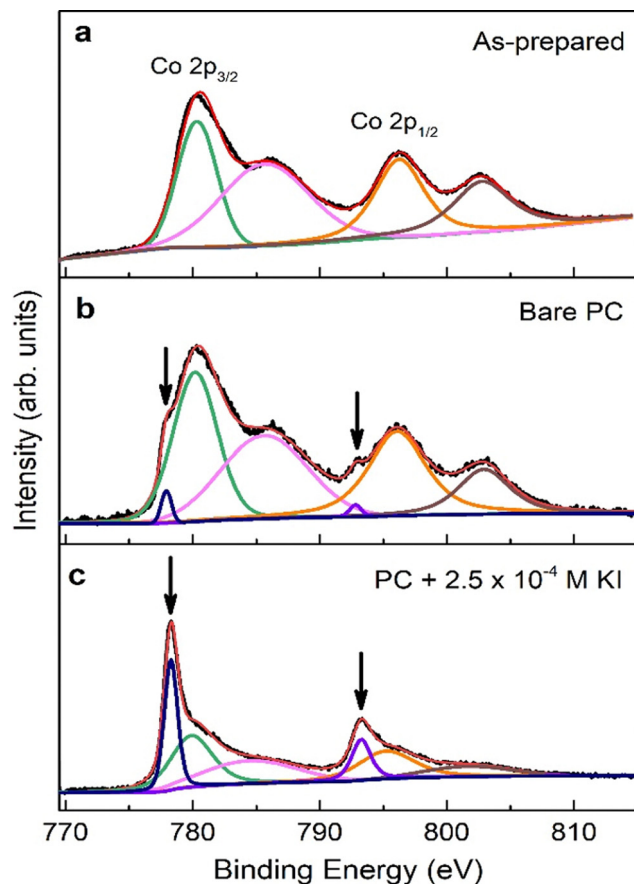
Fig. 5 X-ray photoelectron spectra of Co 2p 3/2 and Co 2p 1/2 for (a) as-prepared, (b) treated in bare PC and (c) PC + 2.5 × 10 −4 M KI samples. The downward arrows point to the Co 2p 3/2 and Co 2p 1/2 peaks of metallic Co (in blue and purple in (b) and (c)). Additionally, green and orange correspond to Co 2+ , and pink and brown to Co 3+ . Solid black lines are experimental data, whereas solid red lines refer to fitting spectra.
