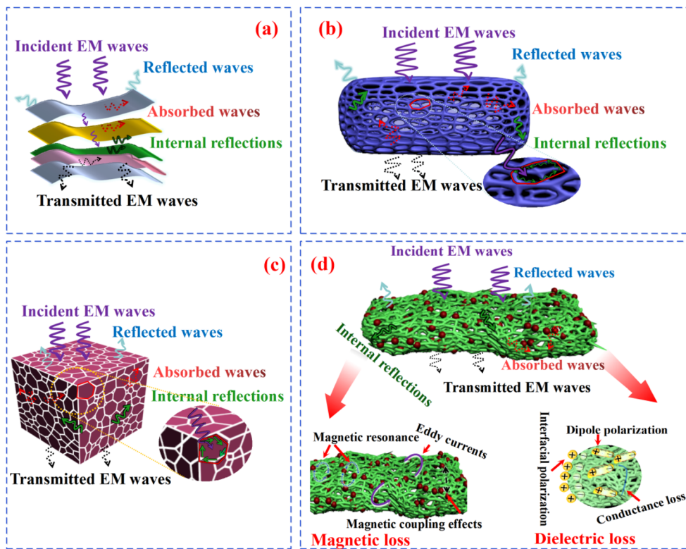
Fig. 3 EMI shielding mechanisms of different structures of MXene/polymer composites: (a) multilayer, (b) porous, (c) segregated, and (d) magnetic/conductive networks.
