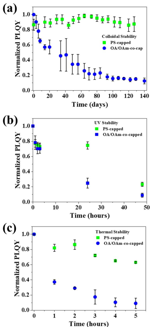
Fig. 5 (a) Colloidal, (b) UV, and (c) thermal (at 80 °C) stabilities of PS-capped and OA/OAm-co-capped CsPbBr 3 PNCs (control sample) synthesized at optimized conditions ( Q_{\text{tol}} = 5000 \text{ mL h}^{-1} and Q_{\text{precursor}} = 60 \text{ mL h}^{-1} ).
