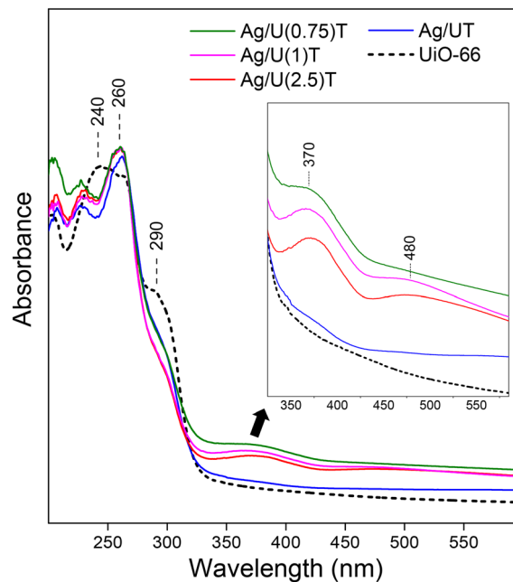
Fig. 4 UV-DRS spectra of thermally-treated Ag/UiO-66 solids obtained with different proportions of silver/citrate. The dotted line shows the spectrum of UiO-66.
