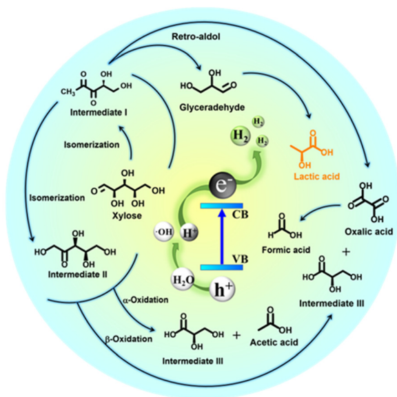
Fig. 8 Possible reaction mechanism of the photocatalytic co-production of hydrogen and lactic acid via RuS 2 @CN-2.
