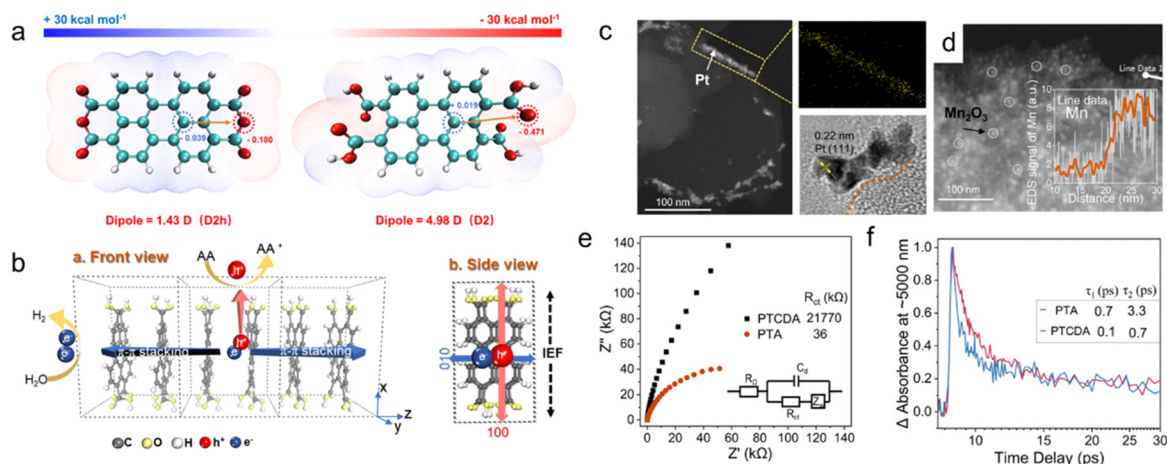
Fig. 3 (a) Molecular dipole calculations. The dipole moment of PTCDA (left) and PTA (right) based molecular electrostatic potential. (b) Schematic diagram of IEF in PTA cell. ADF-STEM photodeposition on PTA with (c) Pt and high resolution and mapping, (d) Mn 2 O 3 (inset: Mn element liner scan). (e) impedance and (f) transient absorption decay kinetics at ~5000 nm of PTCDA and PTA. Reproduced with permission from ref. 45 (Copyright 2022, Springer Nature).
