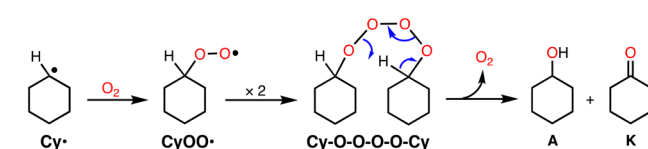
Scheme 2 Russell rearrangement.
