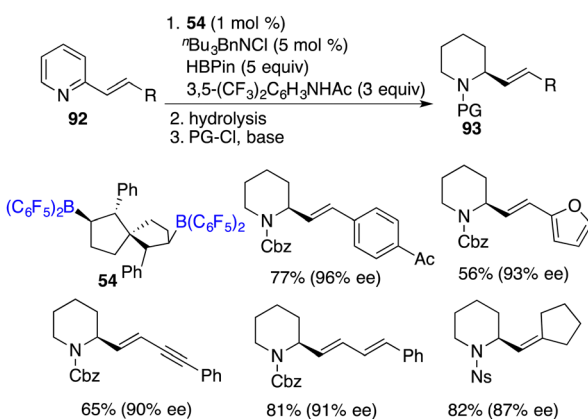
Scheme 52 Metal-free enantioselective reduction of 2-vinylpyridines.
