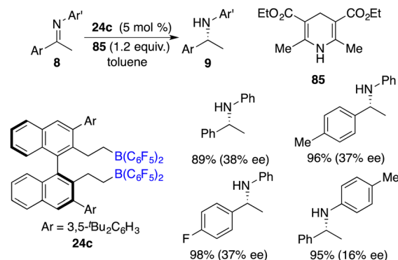
Scheme 49 Asymmetric transfer hydrogenation of imines with Hantzsch esters.
