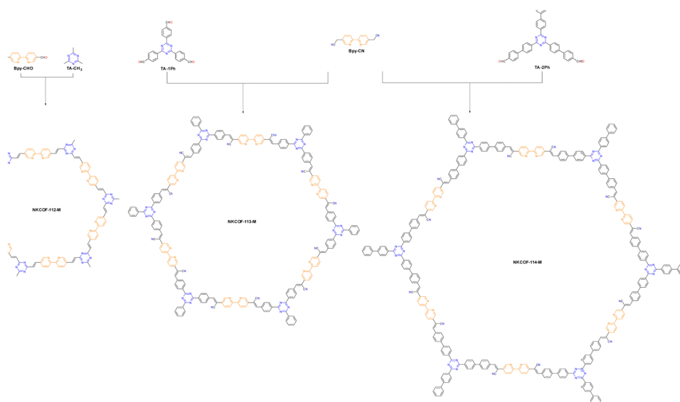
Fig. 5 Synthesis routes and chemical structures of NKCOF-112-M, NKCOF-113-M and NKCOF-114-M. 59
