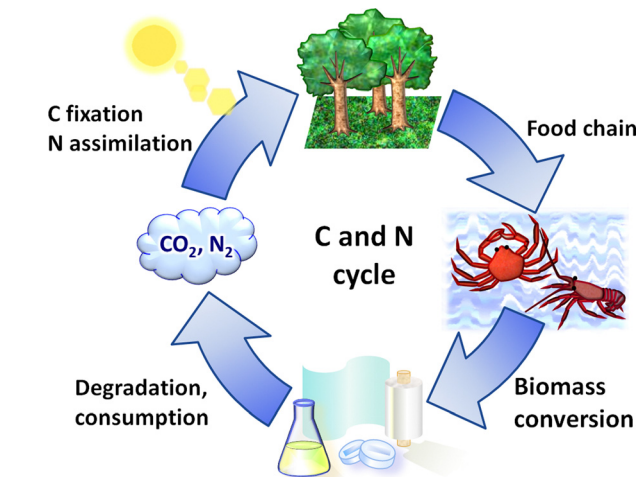
Fig. 2 Nitrogen-containing biorefinery.
