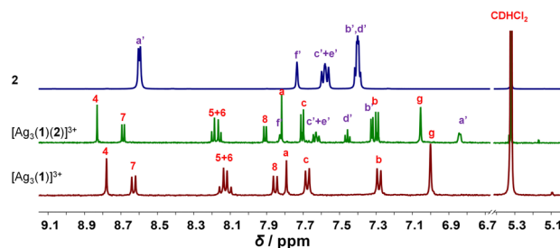
Fig. 1 Partial ^1\text{H} NMR (600 MHz, \text{CD}_2\text{Cl}_2 , 298 K) of silver(i)-loaded deck [\text{Ag}_3(\mathbf{1})(\mathbf{2})]^{\text{3+}} , slider-on-deck [\text{Ag}_3(\mathbf{1})(\mathbf{2})(\mathbf{3})]^{\text{3+}} and biped 2 .
