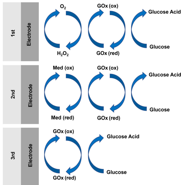
Fig. 9 Schematic illustration of redox mechanisms for the three generations of enzymatic glucose sensor.
