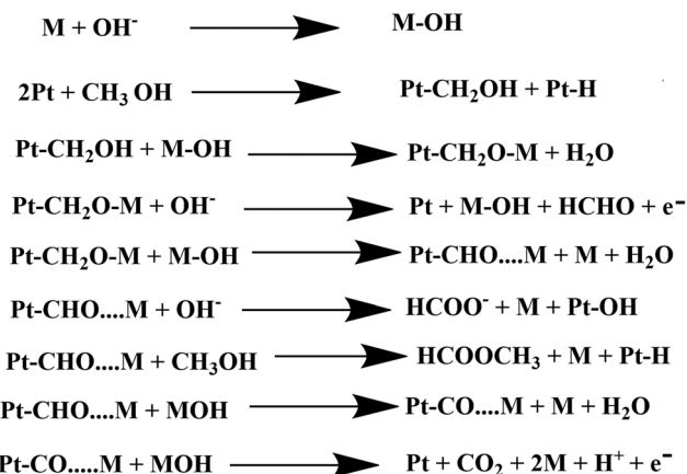
Scheme 2 Electrocatalytic oxidation of methanol by the synthesized heterojunction in the dark condition.
