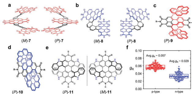
Fig. 4 (a)–(e) Molecular structure of PDI-helicenes (M/P) -7, (M/P) -8, (P) -9, (P) -10, Reproduced with permission from ref. 40. Copyright 2020, American Chemical Society and (P/M) -11; (f) quantitative analysis results of g_R of four (P) -11 OFET devices under CPL irradiations ( \lambda = 635 nm). Reproduced with permission from ref. 41. Copyright 2021, Nature Publishing Group.
