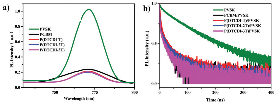
Fig. 4 (a) Steady-state photoluminescence (PL) spectra, and (b) time-resolved photoluminescence (TRPL) decay traces of the perovskite films (PVS) and ETL-covered perovskite films.
