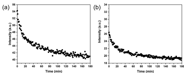
Fig. 4 (a) Change in fluorescence intensity of ARS-loaded MIP particles ( 0.5 \text{ mg mL}^{-1} ) measured after the addition of 1 \text{ M} fructose. (b) Change in fluorescence intensity of ARS-loaded NIP particles ( 0.5 \text{ mg mL}^{-1} ) measured after the addition of 1 \text{ M} fructose. The fluorescence intensity was measured at 560 \text{ nm} in 20 \text{ mM} phosphate buffer.
