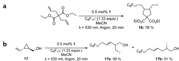
Scheme 4 Radical (a) ring-closing of diethyl 2,2-diallylmalonate and (b) ring-opening of trans -(2-vinylcyclopropyl)methanol via the reductive quenching route of the visible light-mediated ATRA reaction with 1 .
