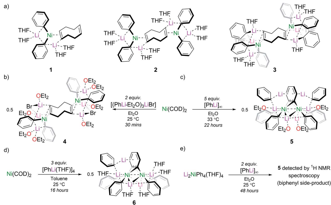
Fig. 1 (a) Lithium nickelates (1–3) derived from Ni(COD) 2 and PhLi; (b) synthesis of [Li 3 (Et 2 O) 4 (LiBr)Ph 2 Ni] 2 COD (4); (c) synthesis of [(PhLi(Et 2 O) 3 LiBr)Ni(COD) 2 ] 2 (5); (d) synthesis of heptametallalithium nickelate 6; (e) observation of 5 by reduction of Li 2 NiPh 4 (THF) 4 .
