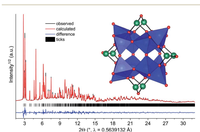
Fig. 7 Difference plot of the final Rietveld refinement for [\text{Ni}(\text{en})_3]_2[\text{As}_8\text{V}_{12}\text{O}_{40}(\text{H}_2\text{O})] \cdot 4\text{H}_2\text{O} with a final R_{\text{wp}} of 4.7% and R_{\text{Bragg}} = 3.7\% . The inset shows the polyhedral representation of the cluster anion in the structure of 2 . Note: the \text{H}_2\text{O} molecule in the cavity of the cluster is not displayed. Blue: \text{VO}_5 polyhedra; green: As; red: O.
